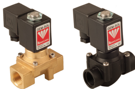
Brass | 1/2" | NC
