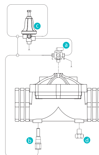
a 3W selector valve b In-line finger filter c Plastic Pilot d Plug
