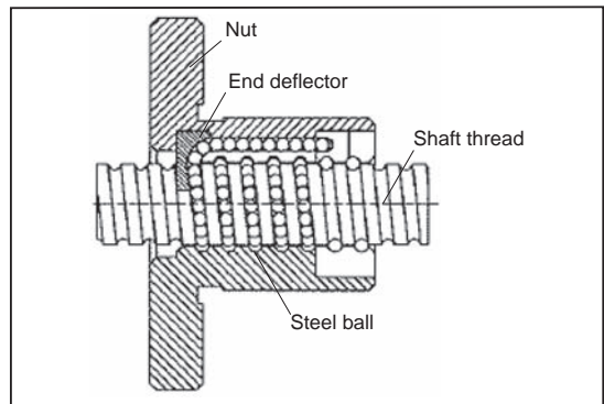
Fig. 12-b End deflector type
