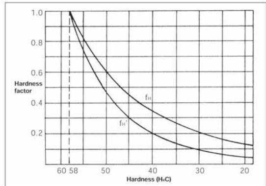
Fig. 27 Hardness factor
