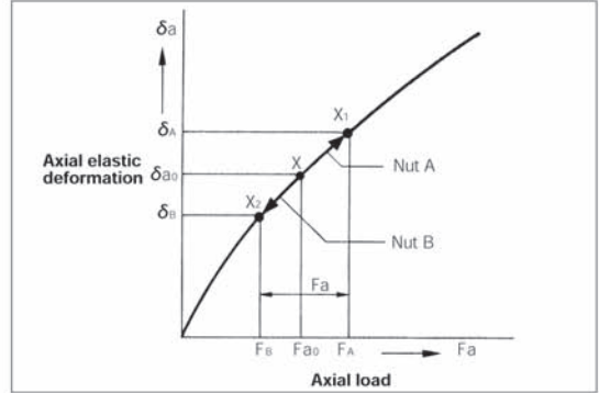
Fig. 23 Axial elastic deformation curves
