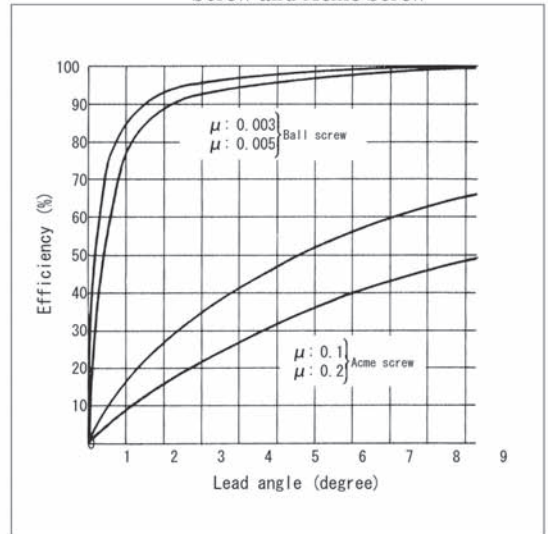
Fig.1 Efficiencies of Ball Screw and Acme Screw
