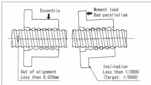
Fig. 13 Unbalanced load
