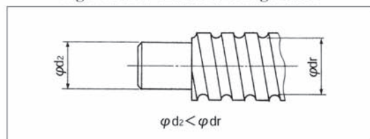
Fig. 10 Screw shaft end configuration
