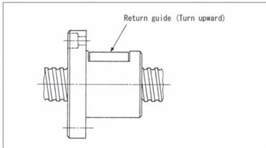
Fig. 14 Mounting direction of return guide type nut
