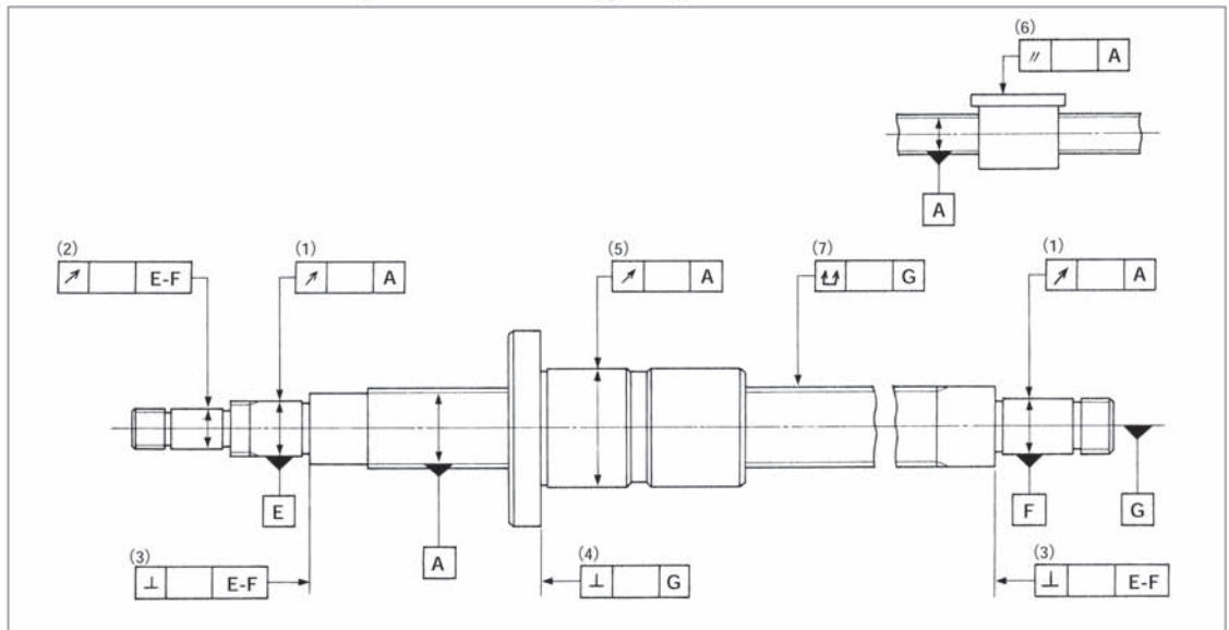
Fig. 4 Accuracies on Supporting Part of Ball Screw
